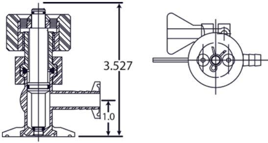
W30 Sample Valve
