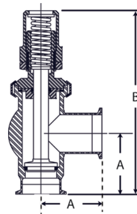
60RTTMP Relief Valve
